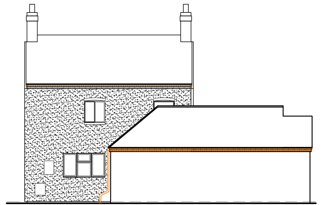
REAR ELEV.
