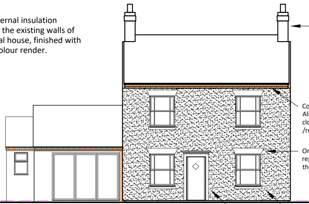
FRONT ELEV.
