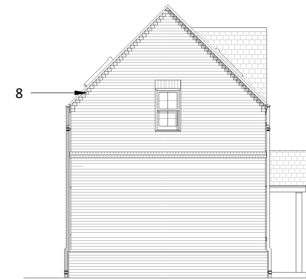
7 South Elevation 1 : 100
