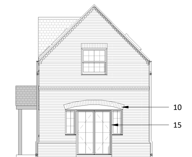
8 North Elevation 1 : 100
