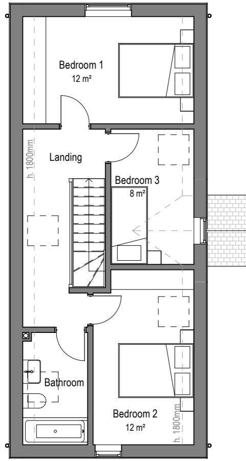
2 First Floor 1 : 100
