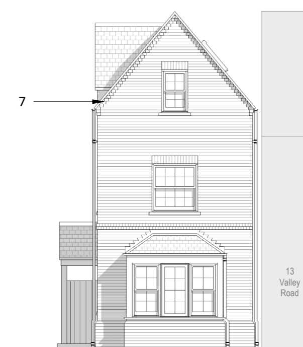
7 South Elevation 1 : 100
