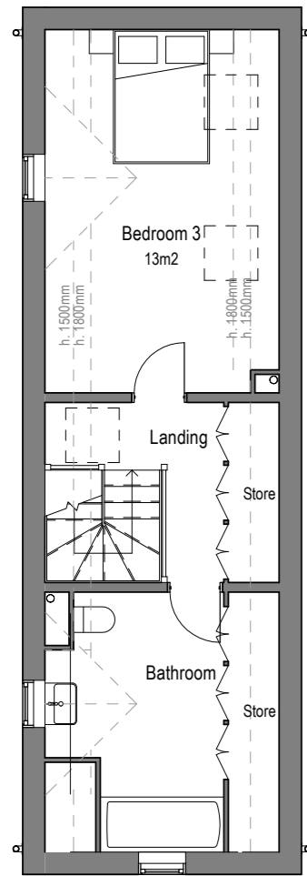
3 Second Floor 1 : 100
