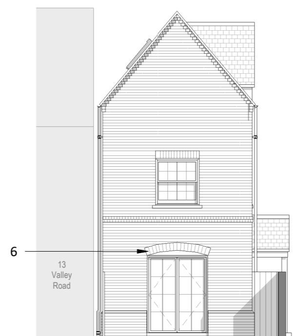
6 North Elevation 1 : 100
