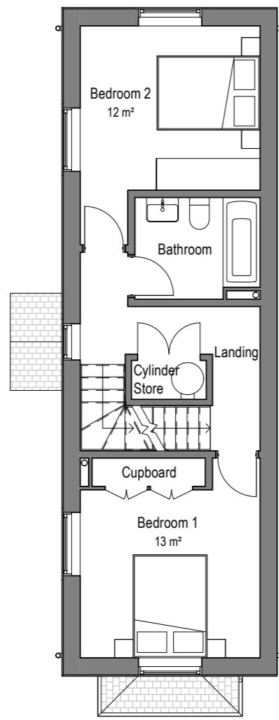
2 First Floor 1 : 100
