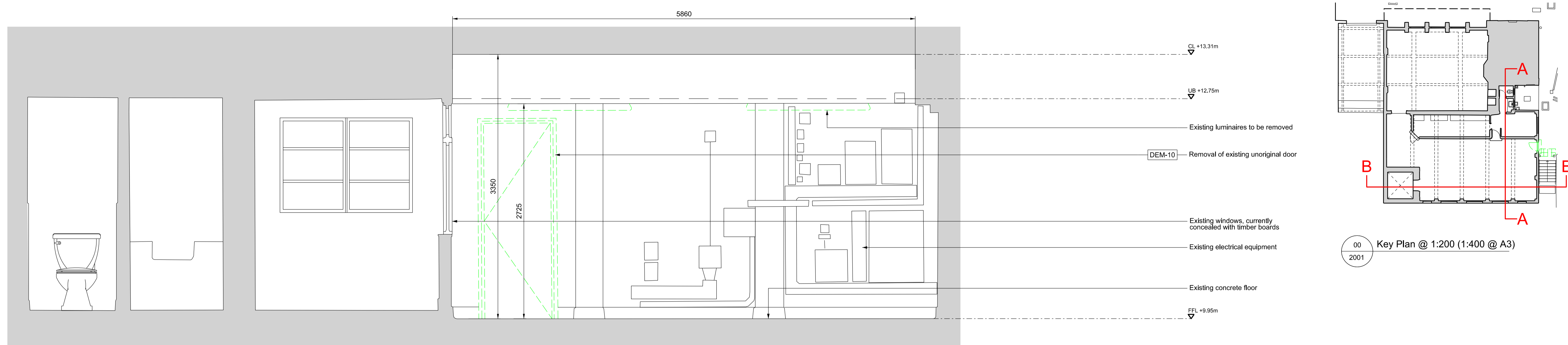
01 Existing Section A-A @ 1:25 (1:50 @ A3) 2001
