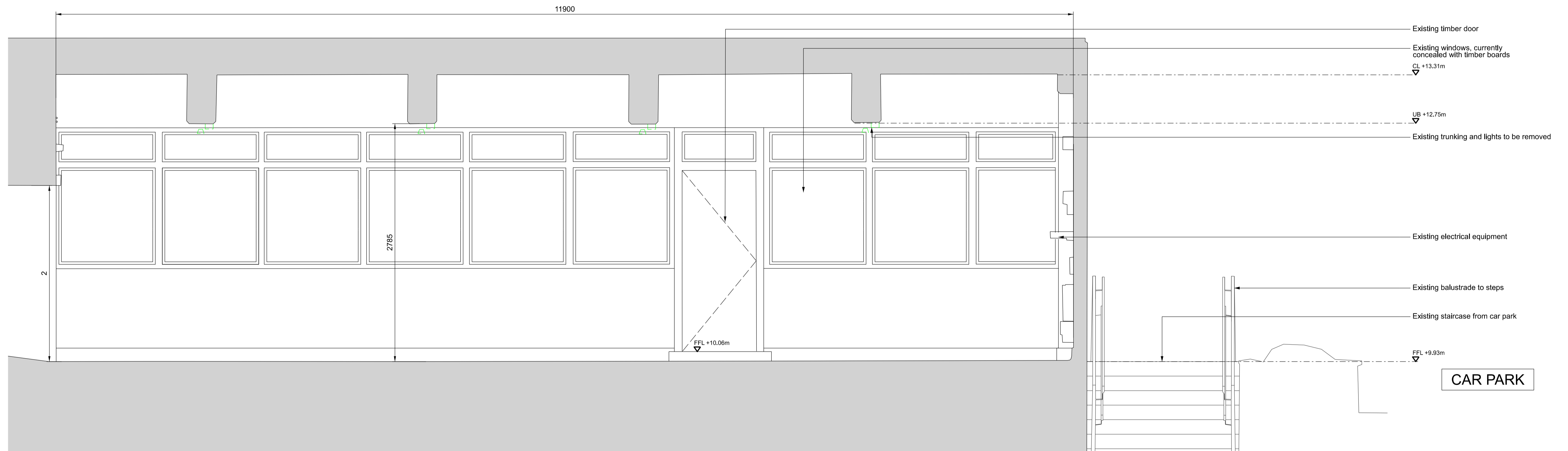
02 Existing Section B-B @ 1:25 (1:50 @ A3) 2001
