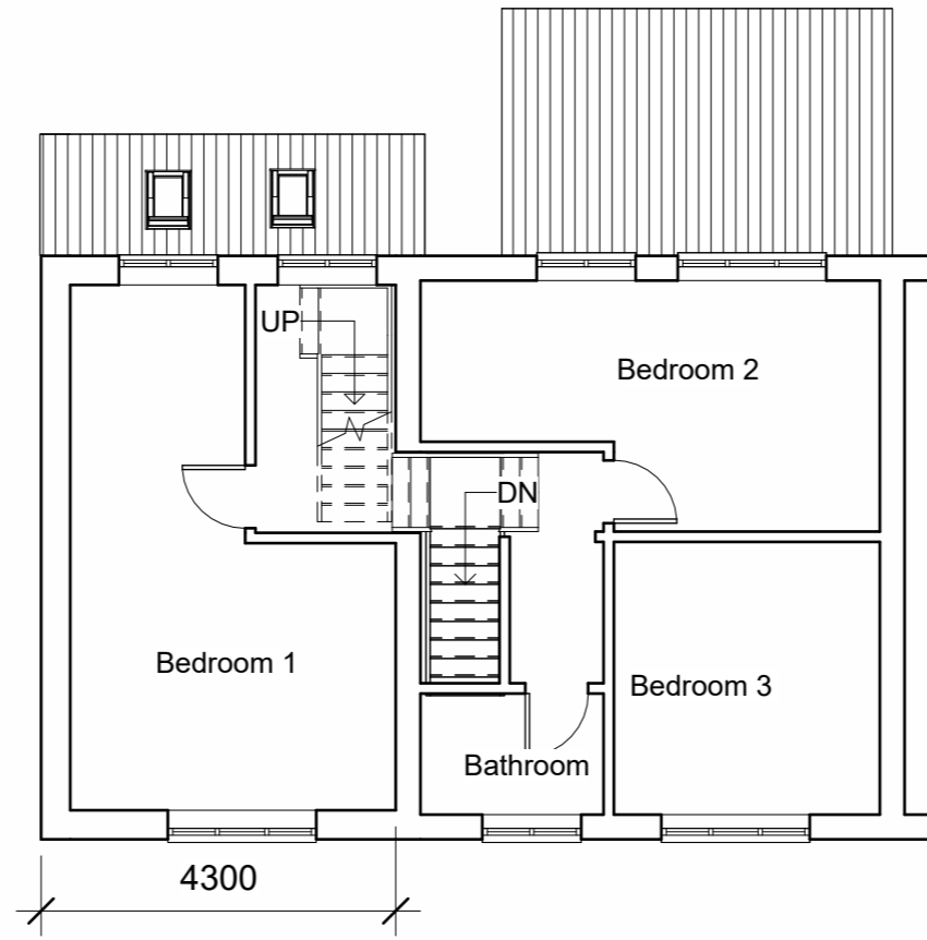
2 Proposed First Floor 1 : 100
