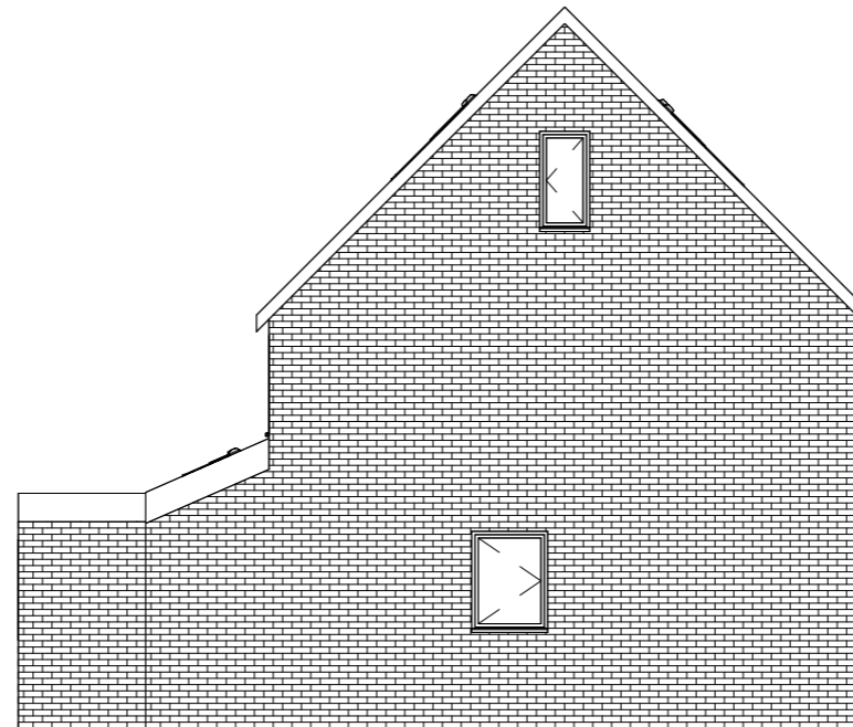
4 Proposed Side B Elevation 1 : 100
