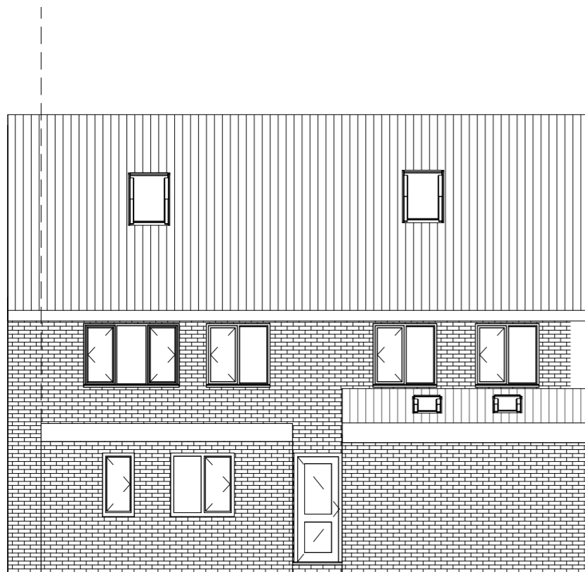
2 Proposed Rear Elevation 1 : 100
