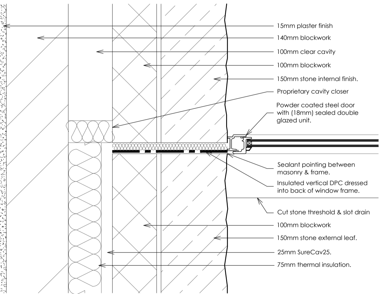
Door Jamb to Masonry Detail - 1:5
