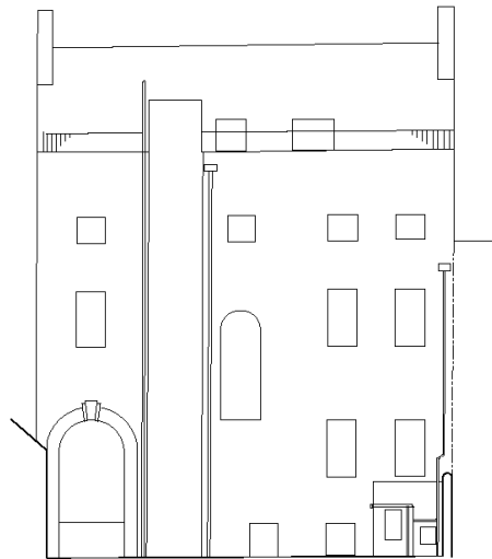
3 008 EXISTING WEST ELEVATION
