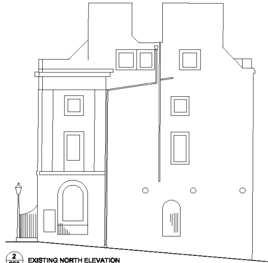
2 008 EXISTING NORTH ELEVATION
