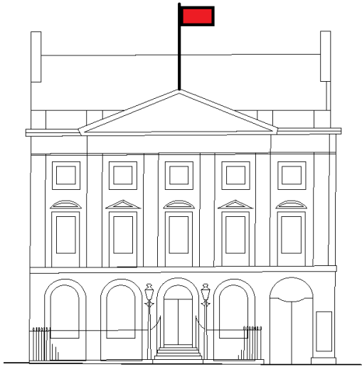
1 008 EXISTING EAST ELEVATION
