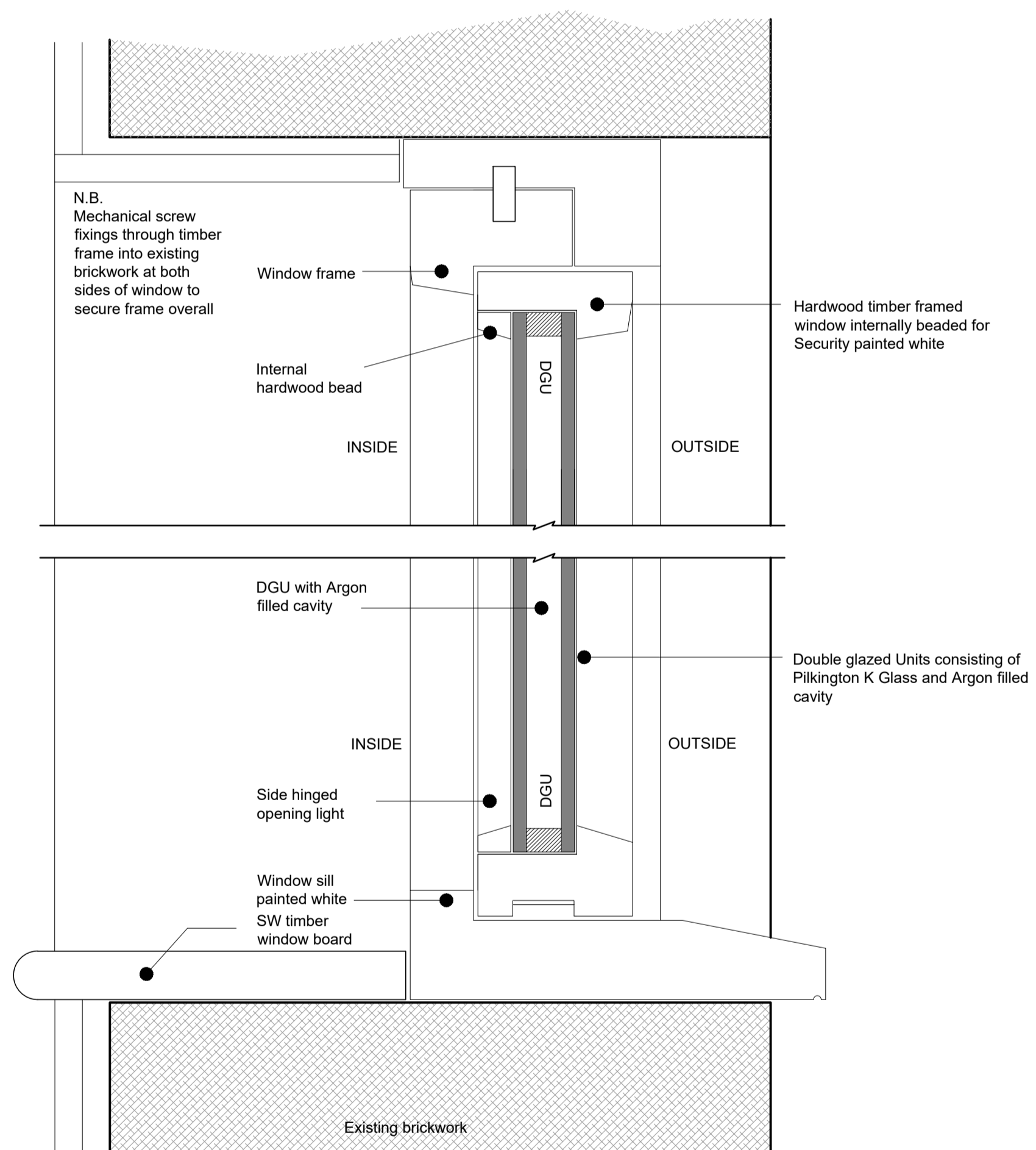
Side opening Window - Section Thru Scale - 1:2
