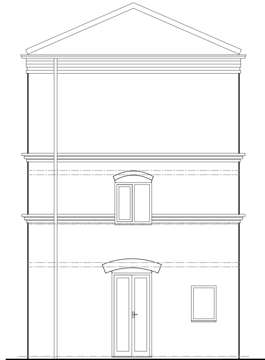
ELEVATION - EAST
