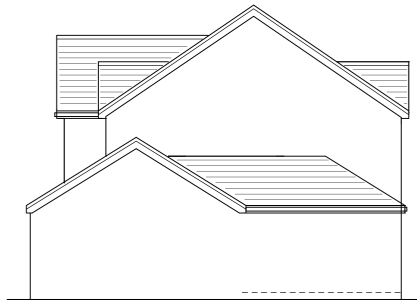
right side (southwest) elevation
