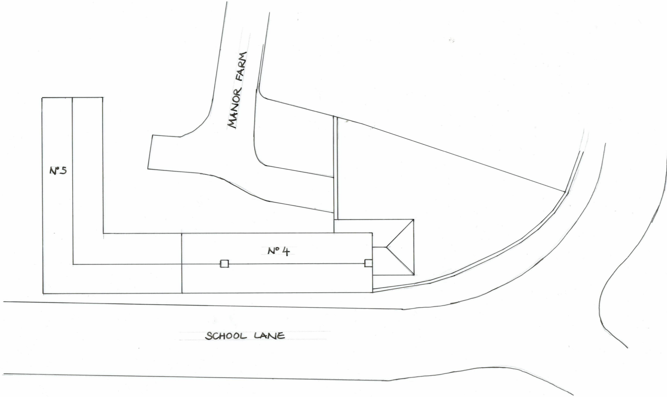
EXISTING SITE LAYOUT 1:200
