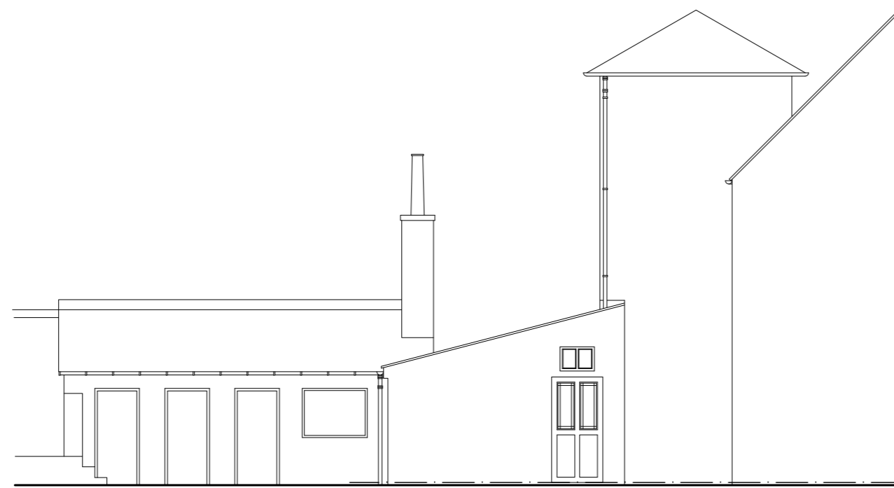
SIDE ELEVATION (WEST) scale 1:100
