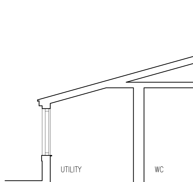
EXISTING CROSS SECTION A-A Scale 1:50
