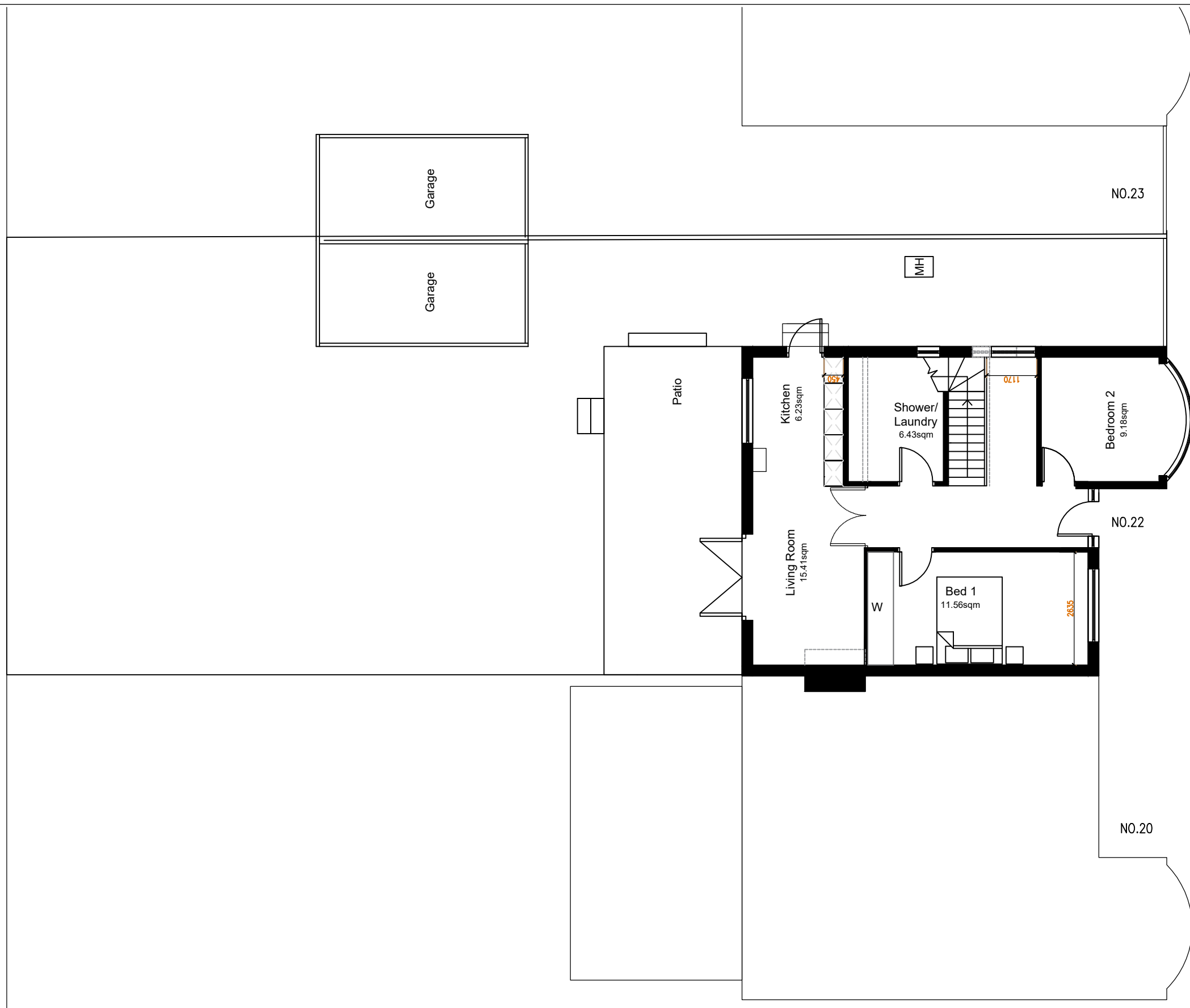
PROPOSED BLOCKPLAN
