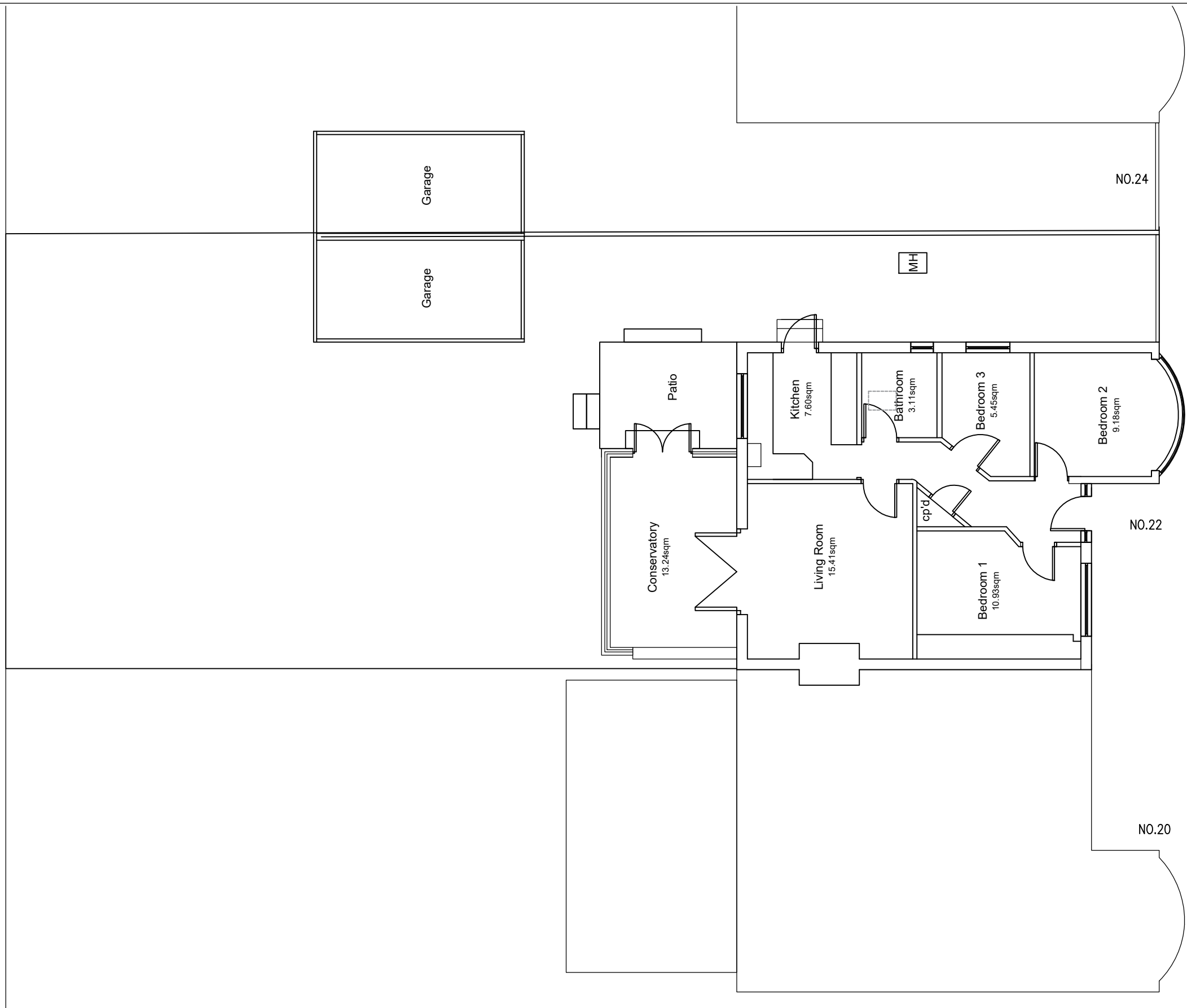
PRE-EXISTING BLOCKPLAN
