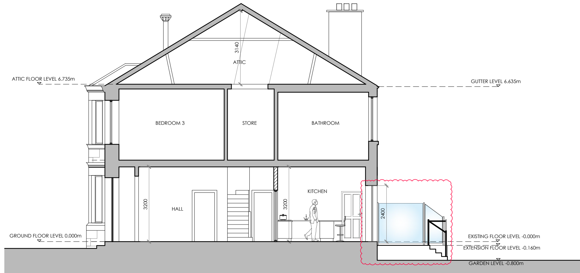
SECTION AA AS PROPOSED
