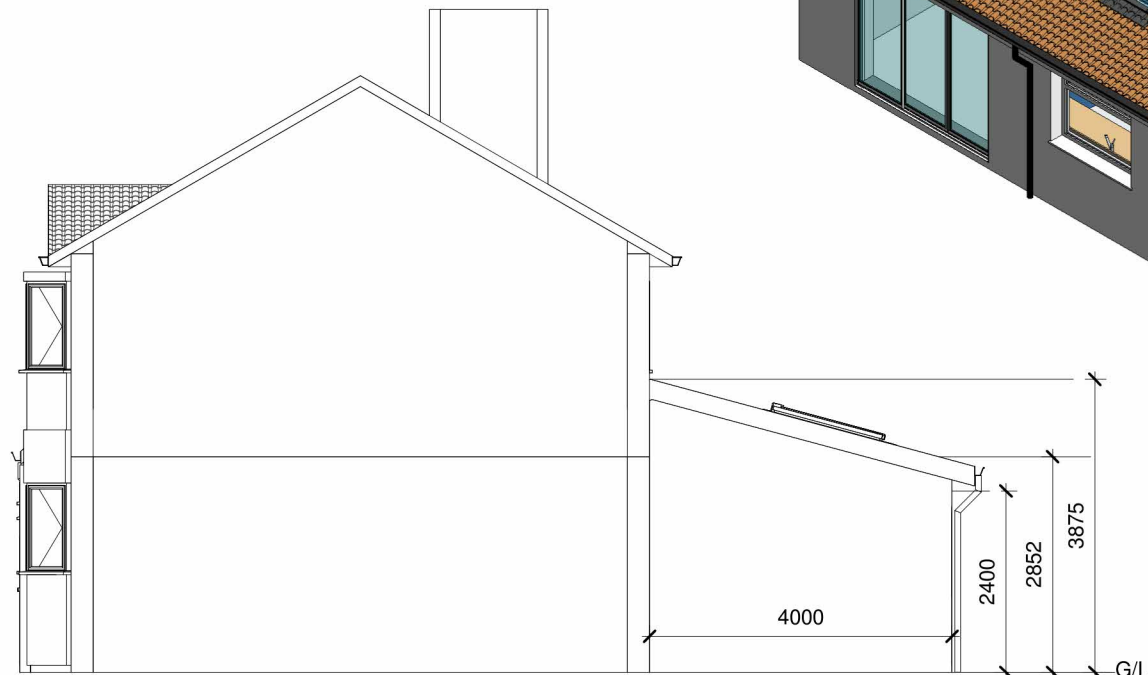
4 Proposed Side Elevation B 1 : 100
