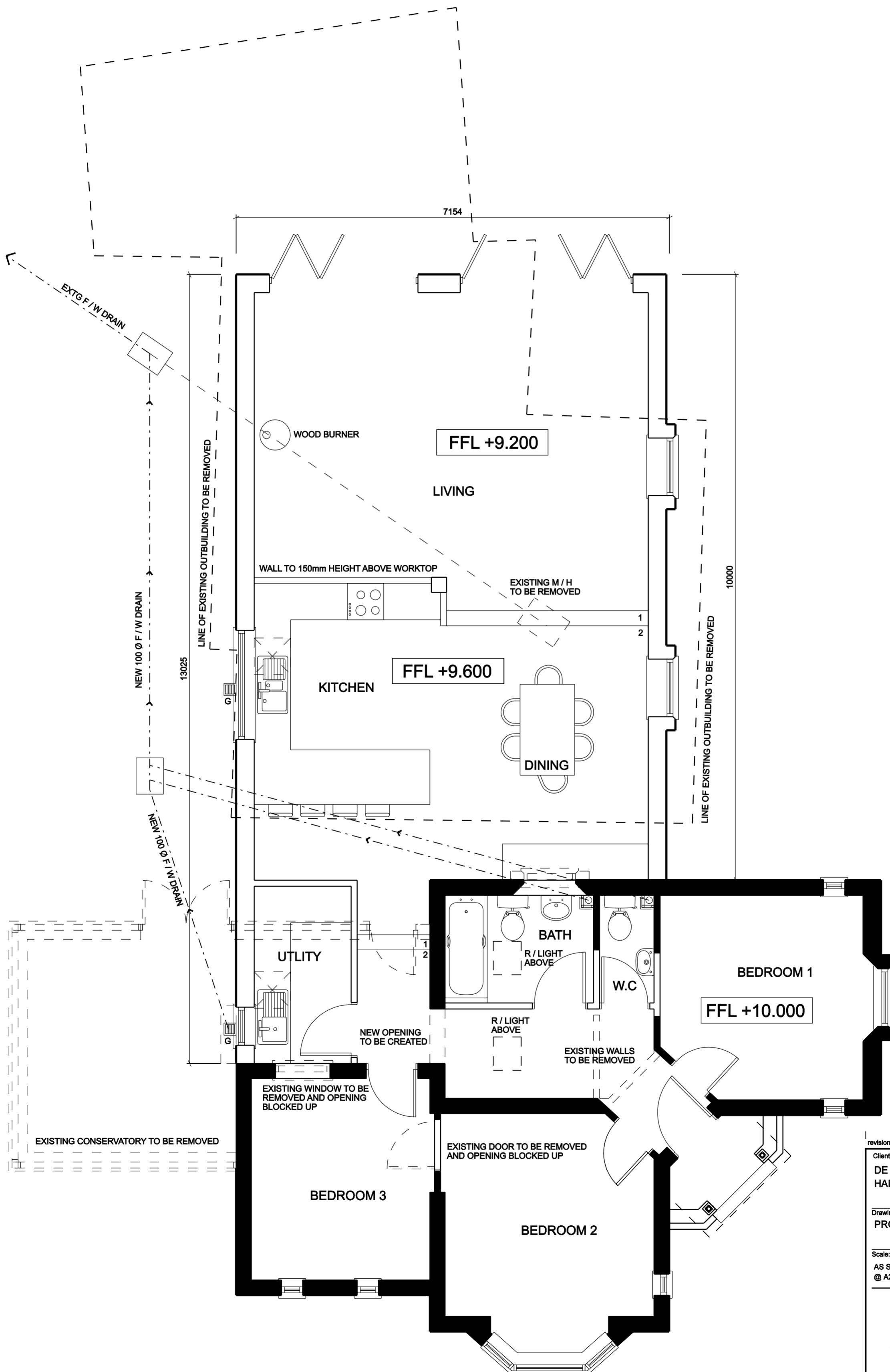
PROPOSED FLOOR PLAN (SCALE - 1:50)
