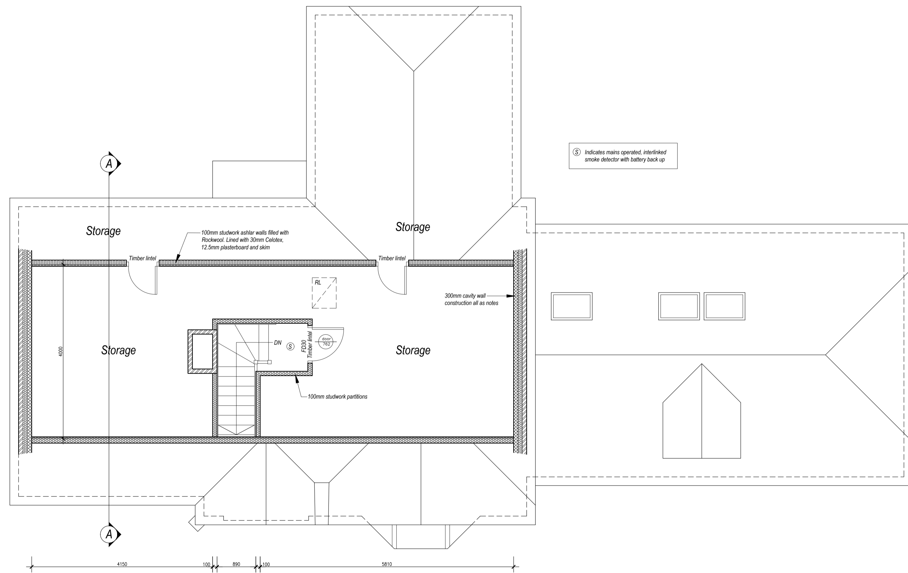
Proposed Second Floor Plan Scale: 1:50
