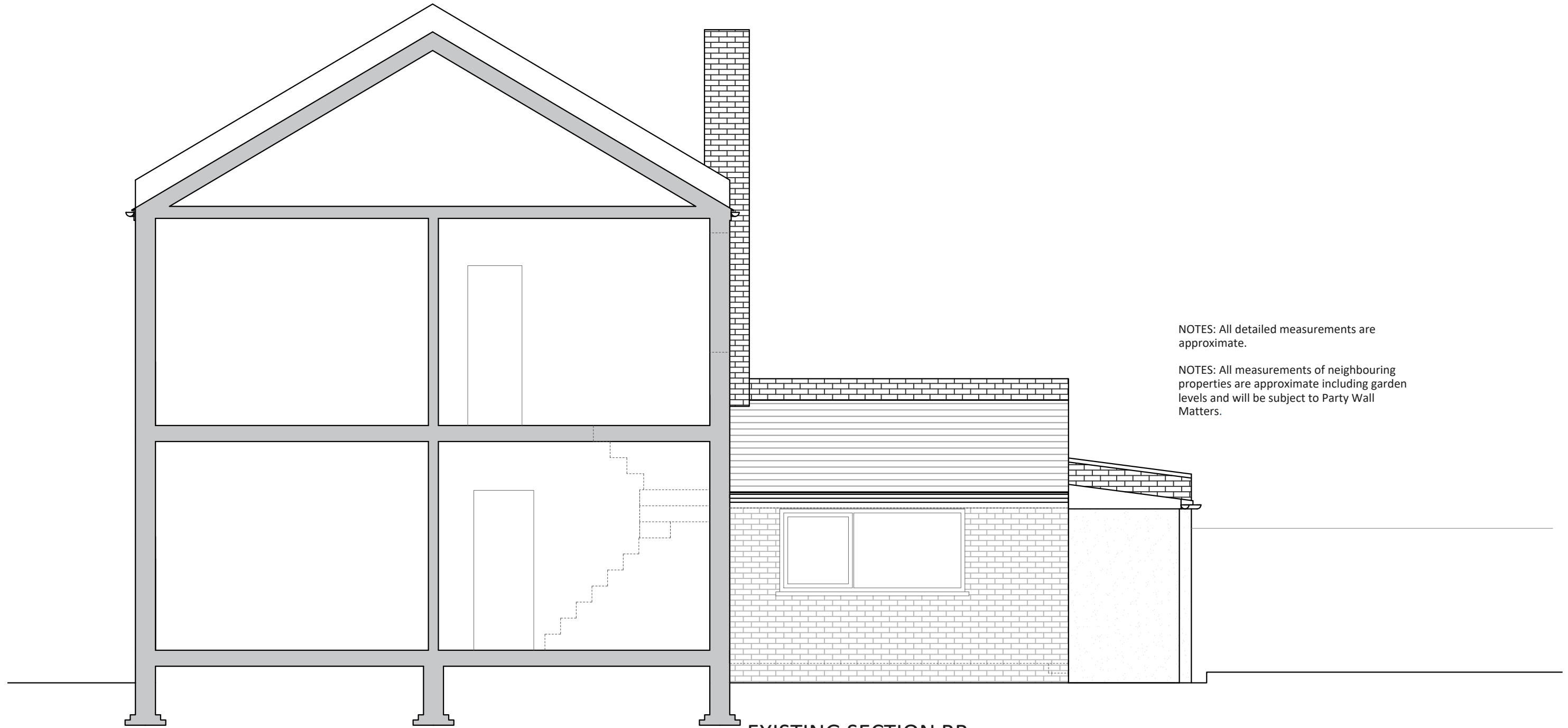
EXISTING SECTION BB SCALE 1:50
