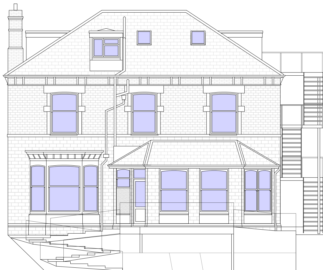
EXISTING REAR (EAST) ELEVATION
