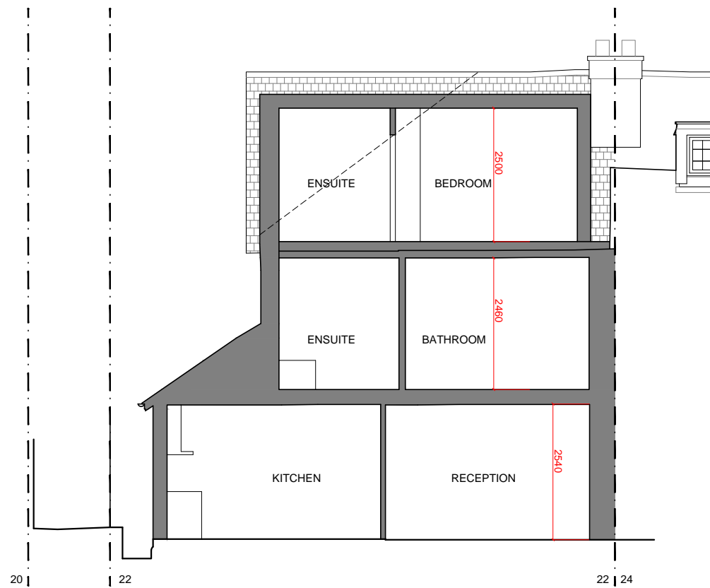
SECTION CC
