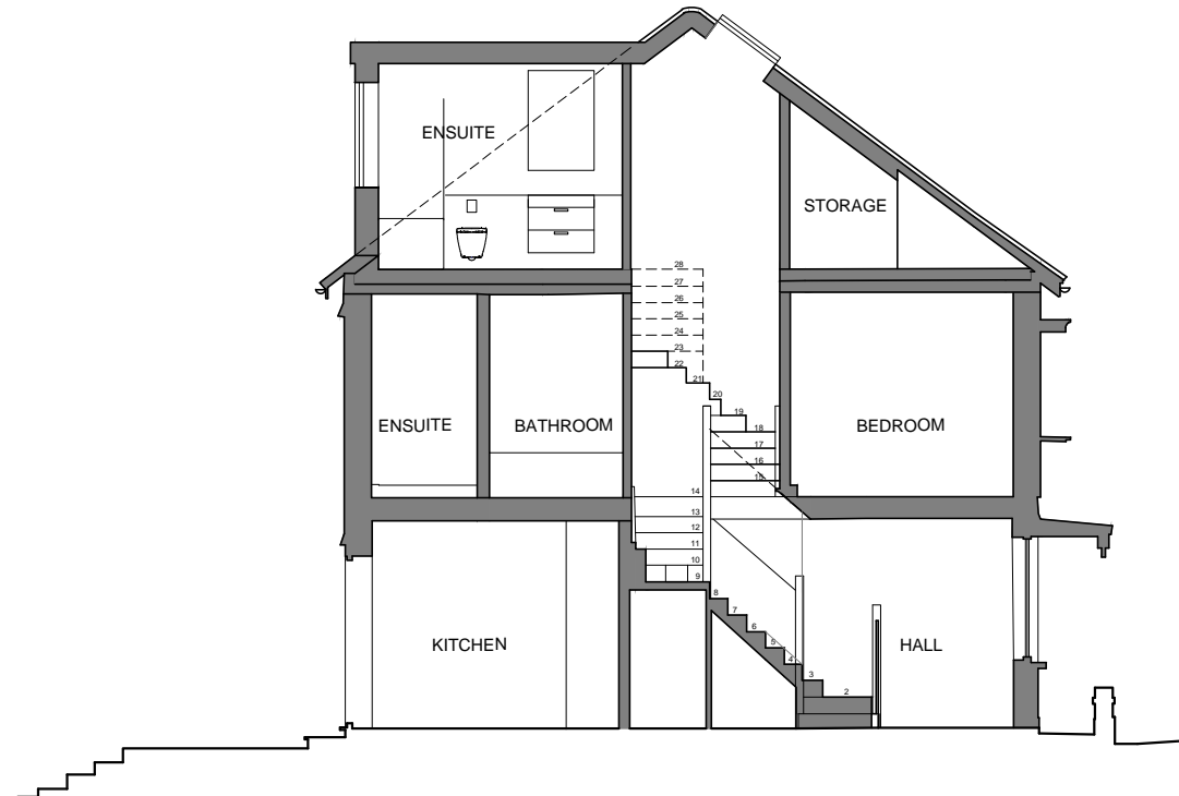
SECTION BB
