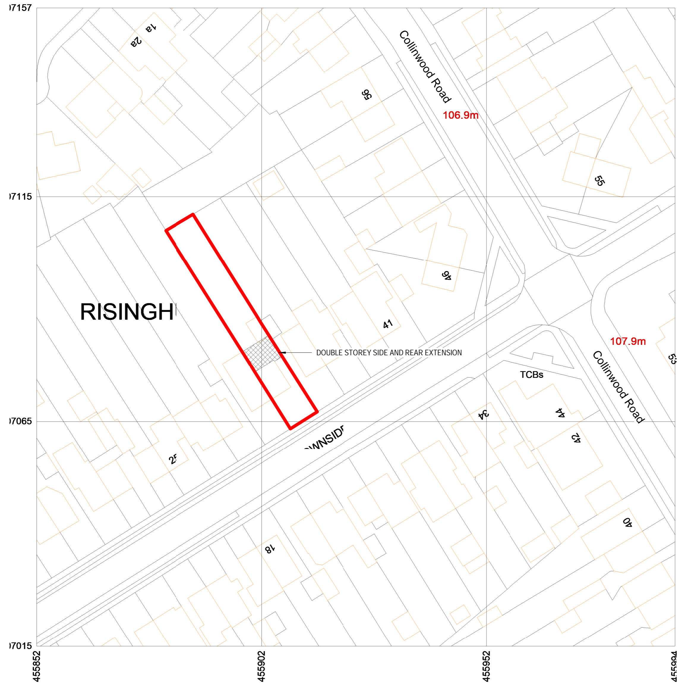
1 S-P4-Proposed- Block Plan 1 : 500
