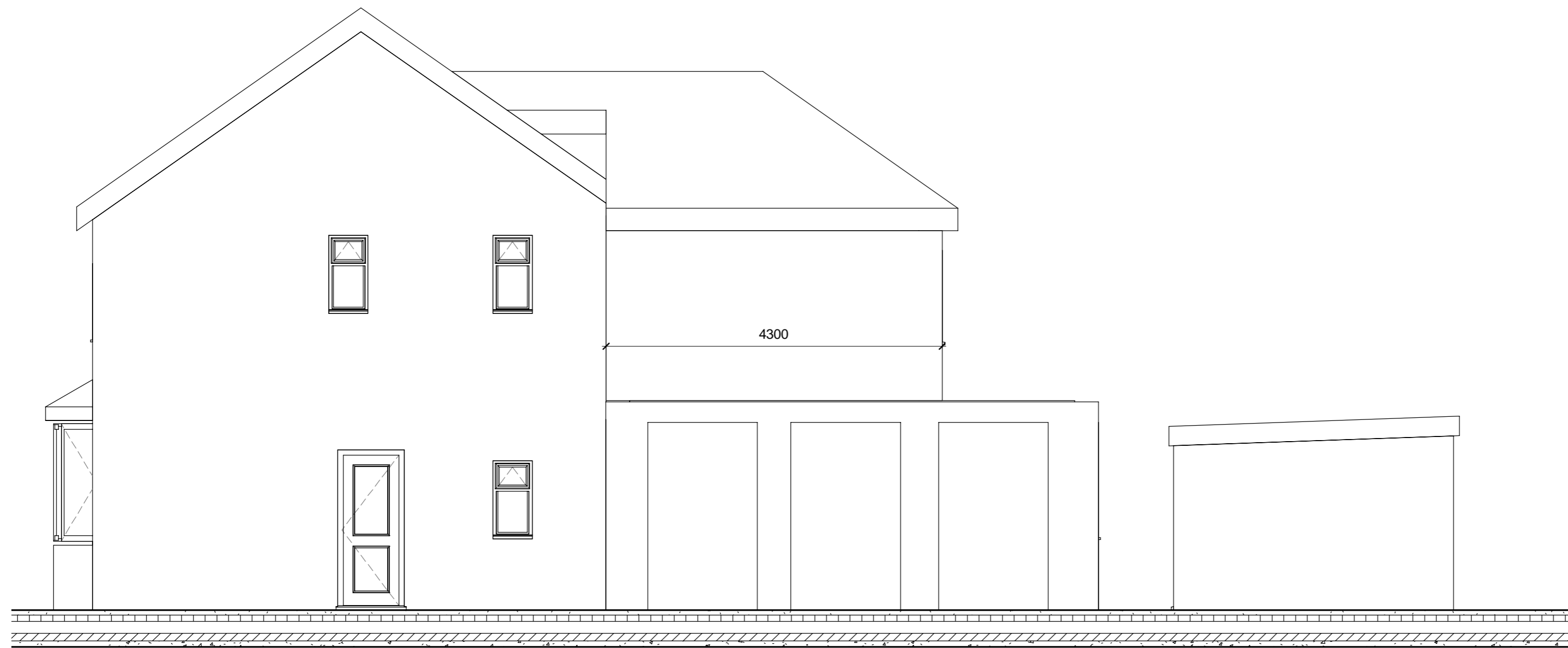
1 P4-Proposed Side Elevation from no.35 1 : 50
