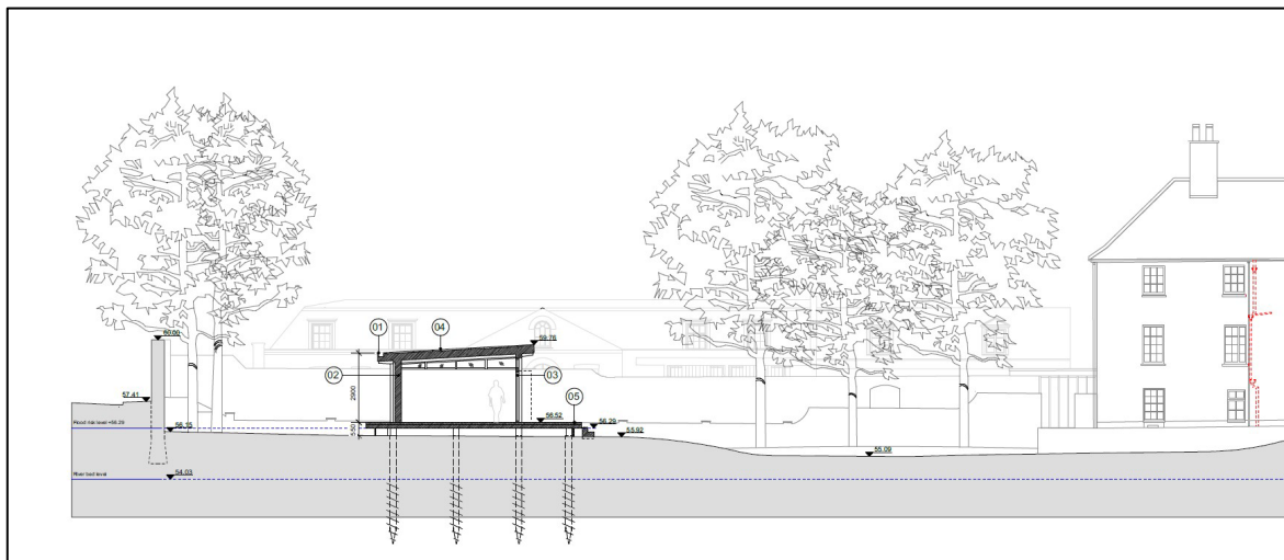
Extract from plan GH(20)A16-Proposed Boat House Section
