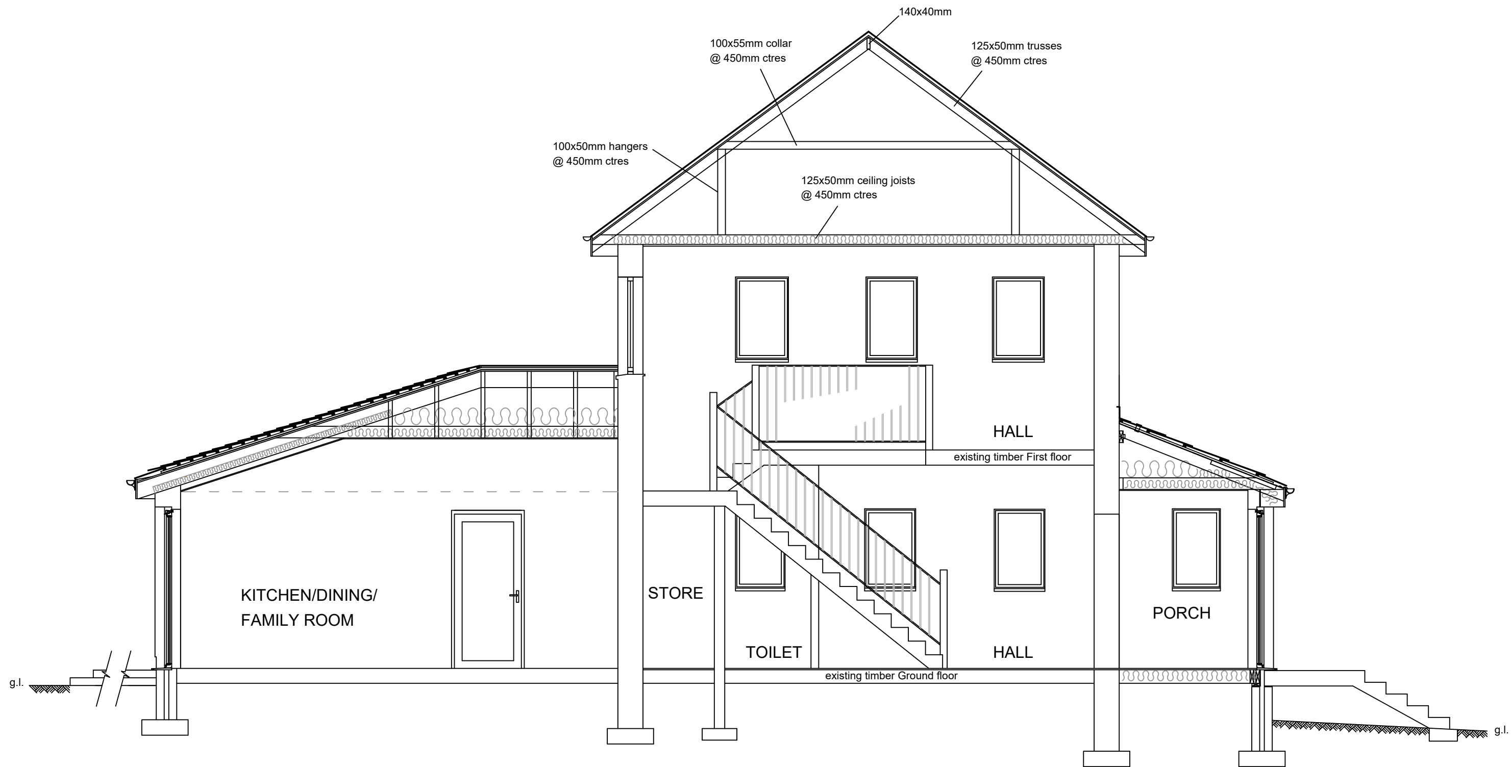
SECTION THRO' A-A (EXISTING)
