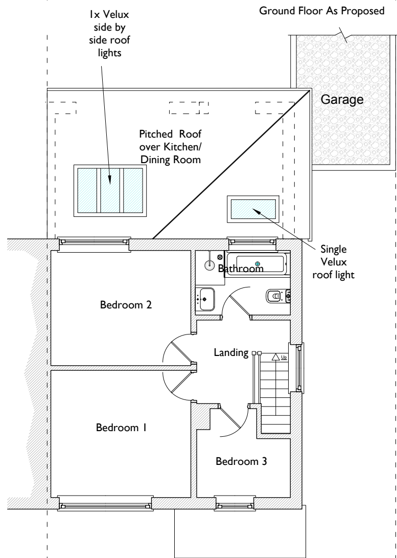
First Floor As Proposed
