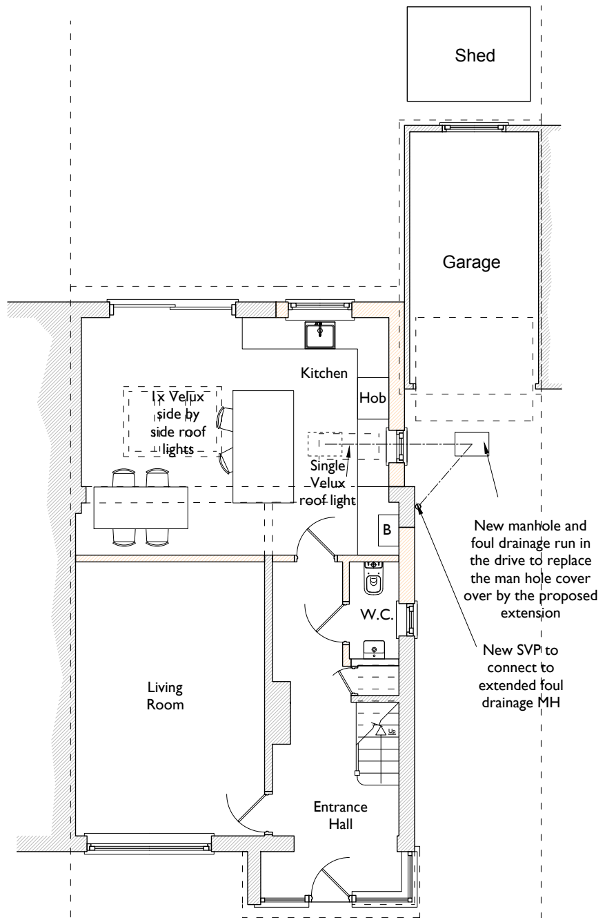
Ground Floor As Proposed
