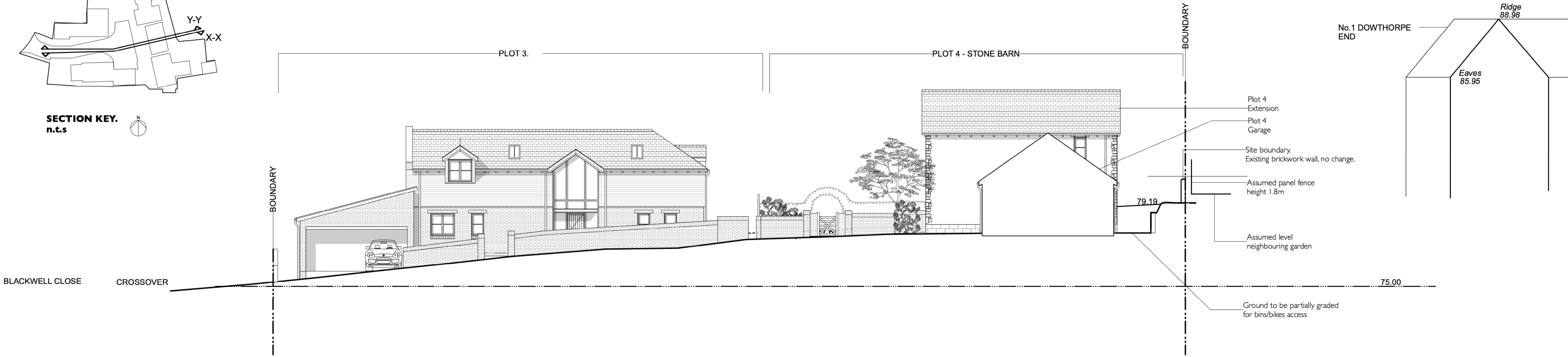
Y-Y OUTLINE SITE SECTION - East to West through shared surface road, looking north
