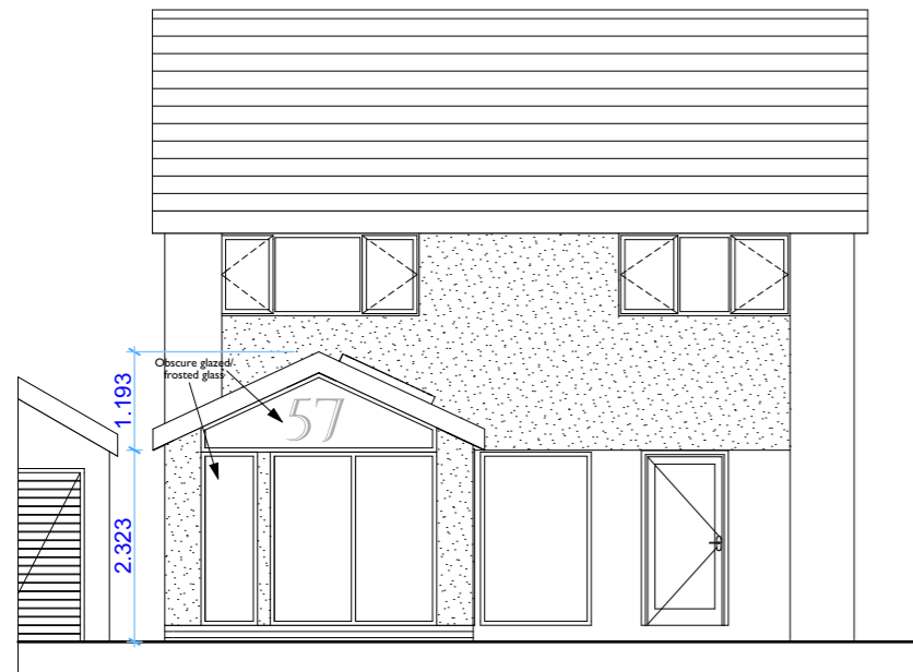
FE1 Front Elevation 1:100
