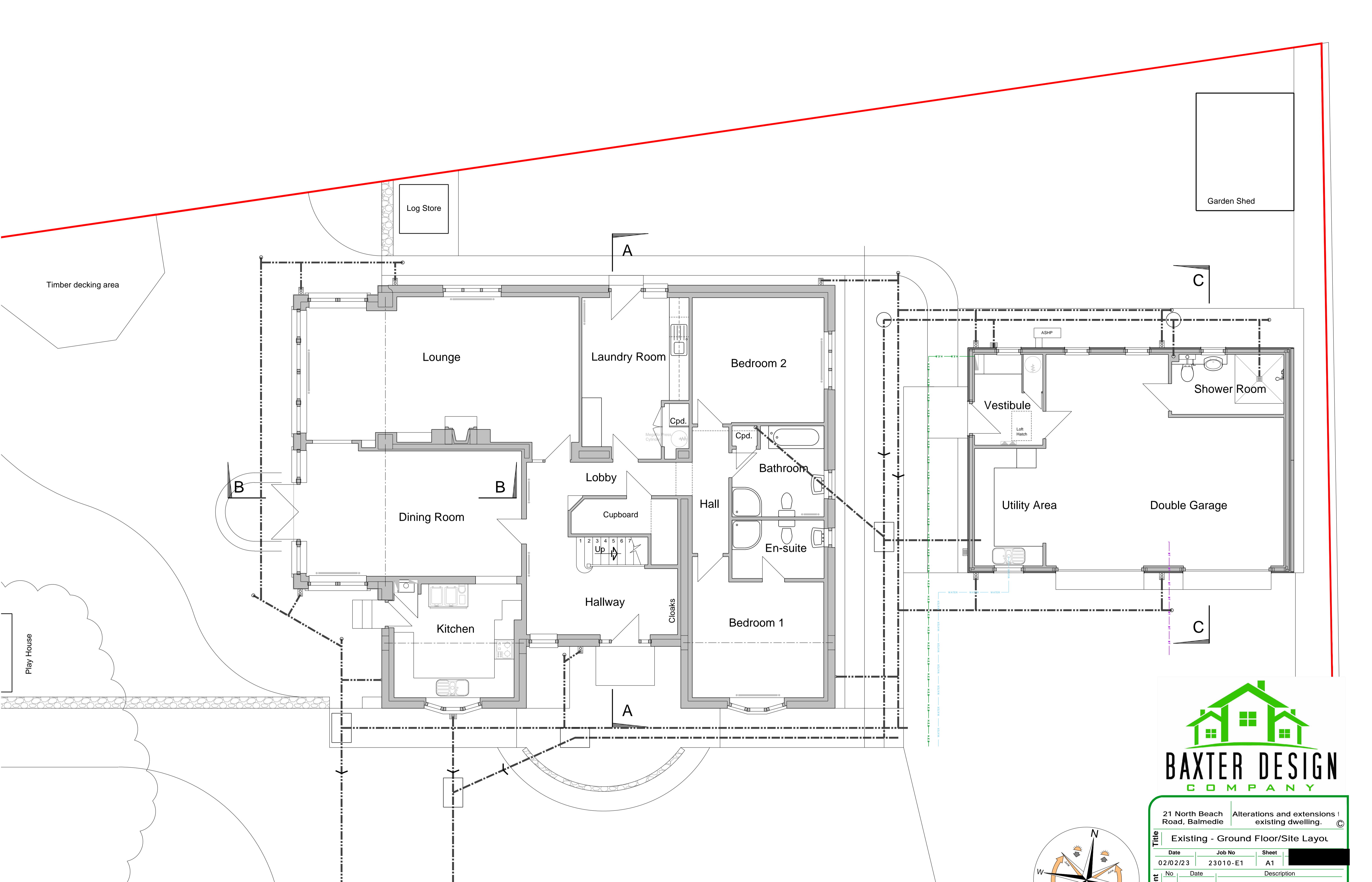
Ground Floor Layout Plan : Scale 1 : 50
