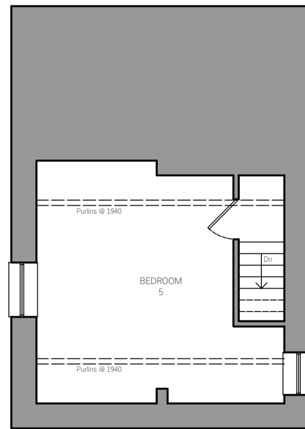
PROPOSED LOFT PLAN 1:100
