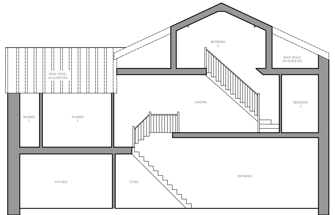
PROPOSED CROSS-SECTION 1:100
