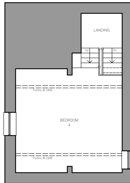
EXISTING LOFT PLAN 1:100
