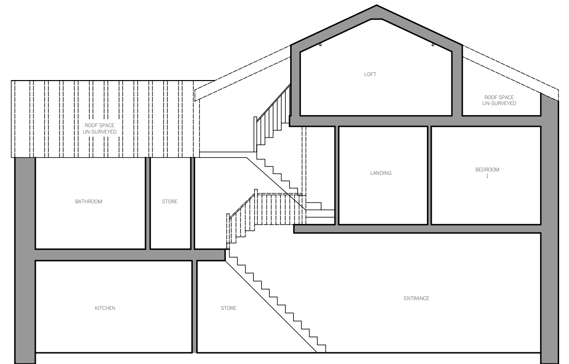
EXISTING CROSS-SECTION 1:100
