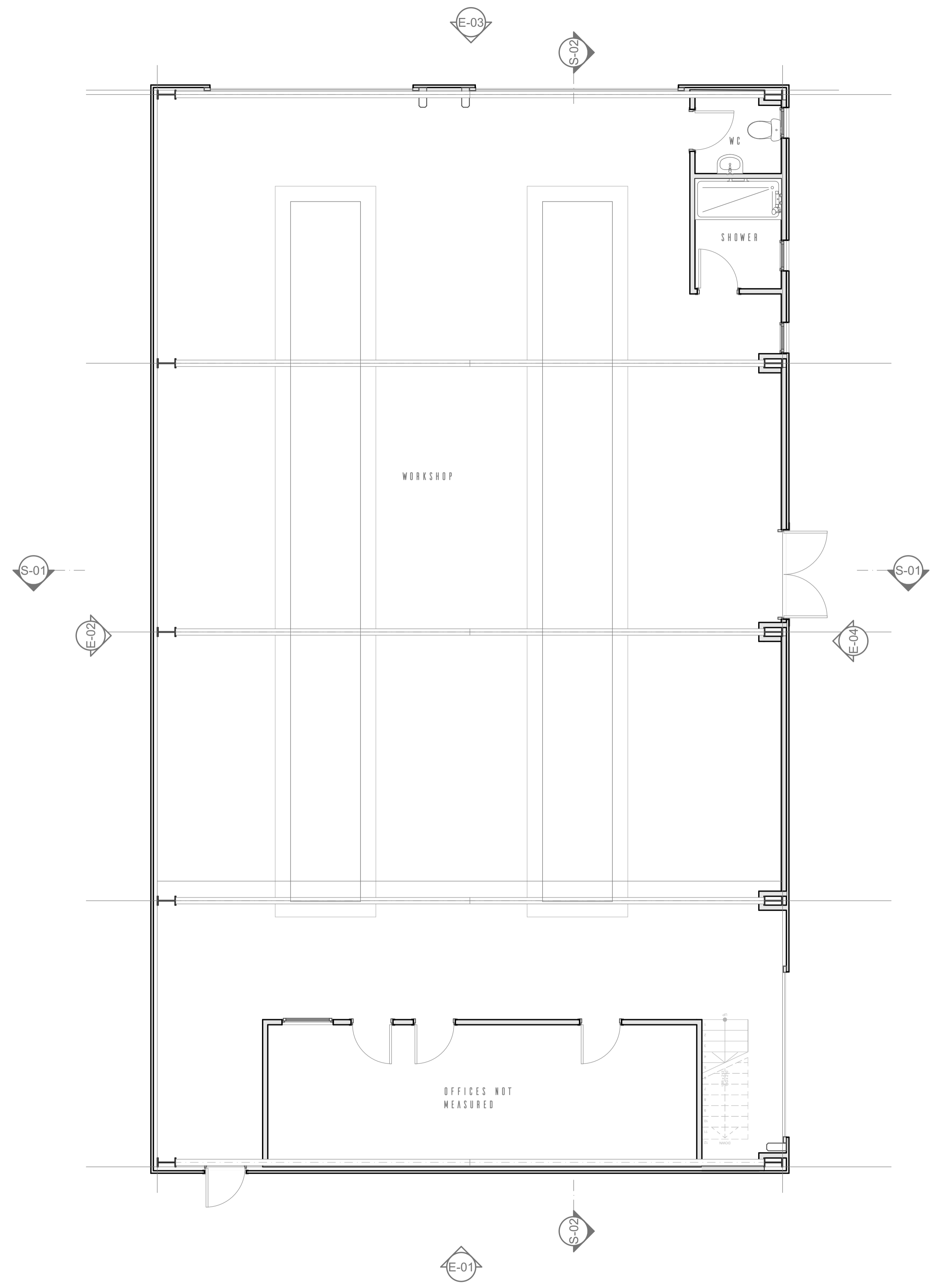
GF-Ground Floor 1:50
