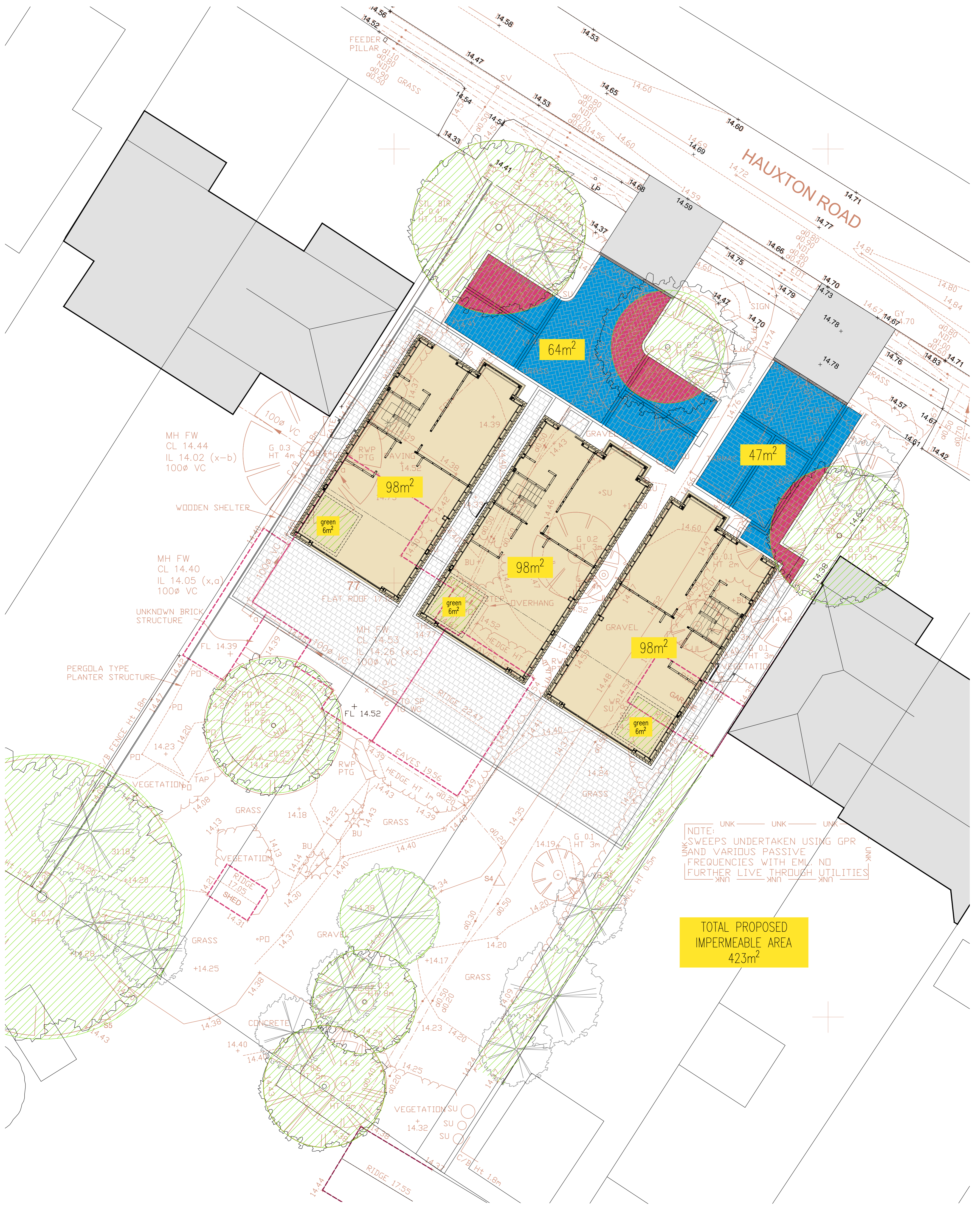
PROPOSED IMPERMEABLE AREAS PLAN (SCALE 1:100)
