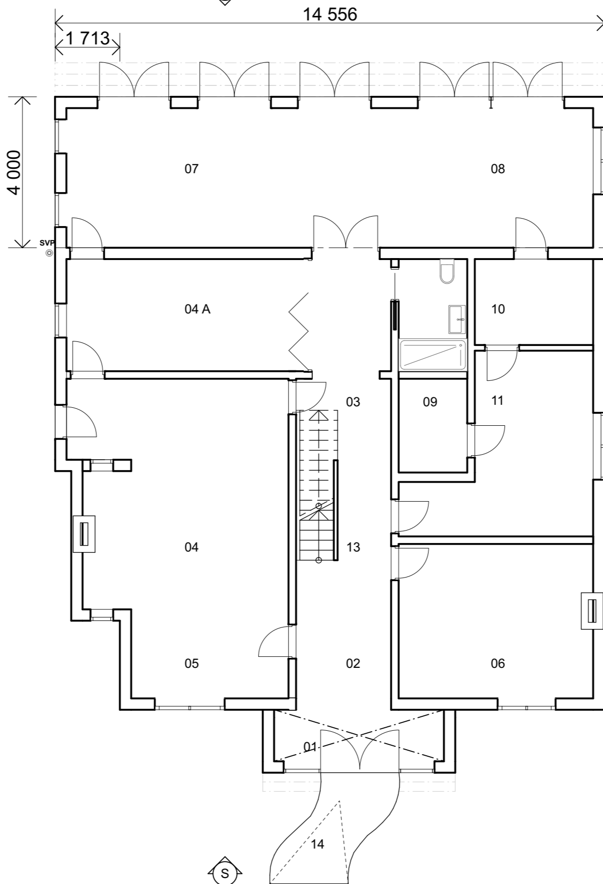
GF-Ground Floor
