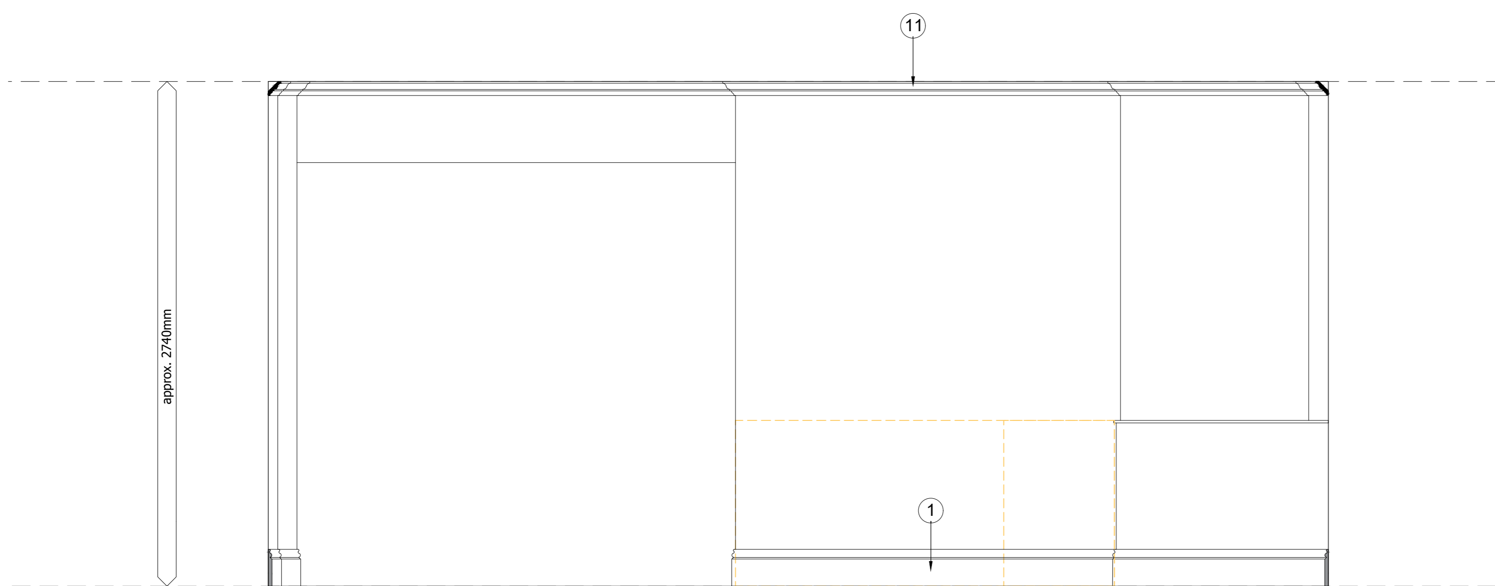
4 ELEVATION SCALE 1:20
