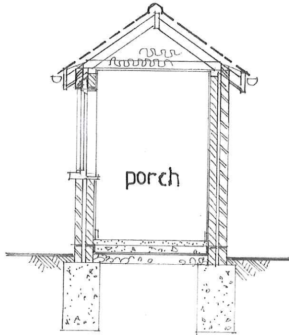
TYPICAL SECTION
