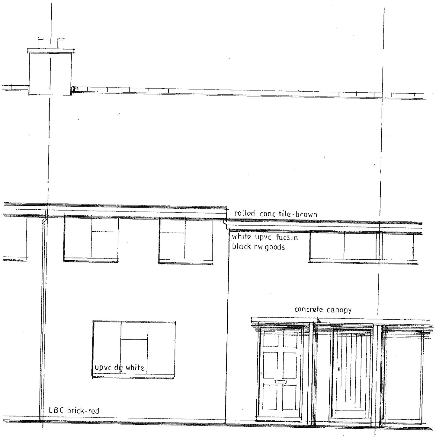
EXISTING FRONT ELEVATION 1/50
