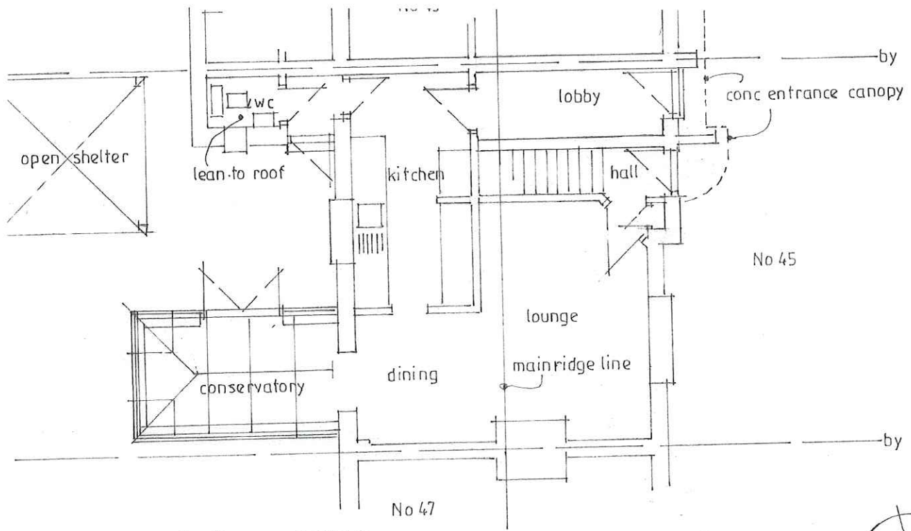
ex. ground floor 1/100
