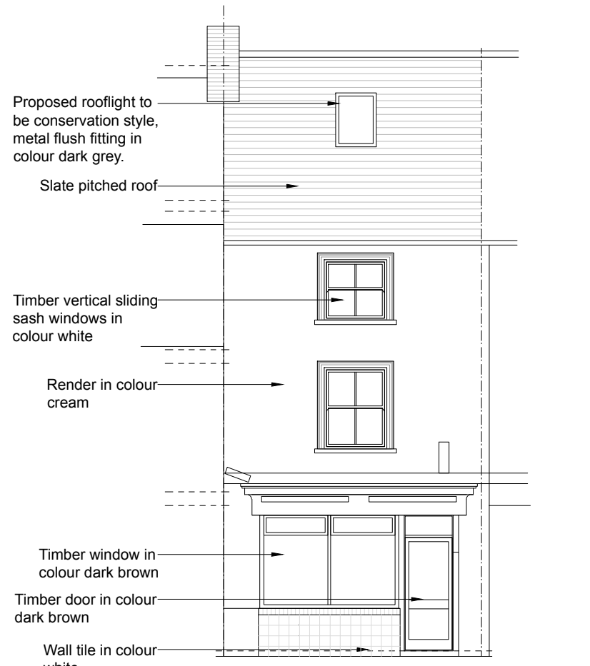
Front (North) Elevation as proposed
