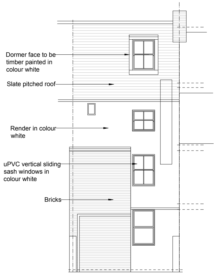
Rear (South) Elevation as proposed
