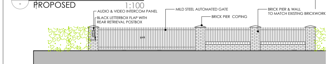
2 FRONT BOUNDARY WALL/GATE PROPOSED
