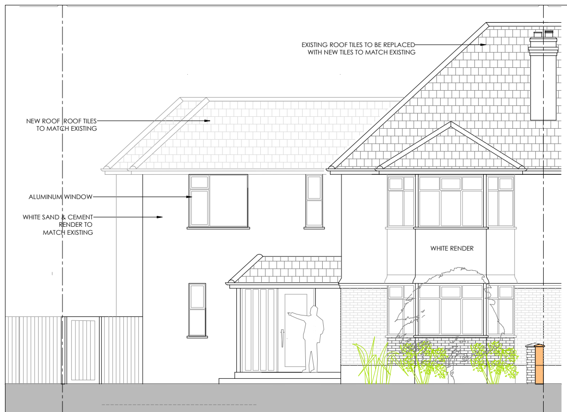
1 FRONT ELEVATION PROPOSED
