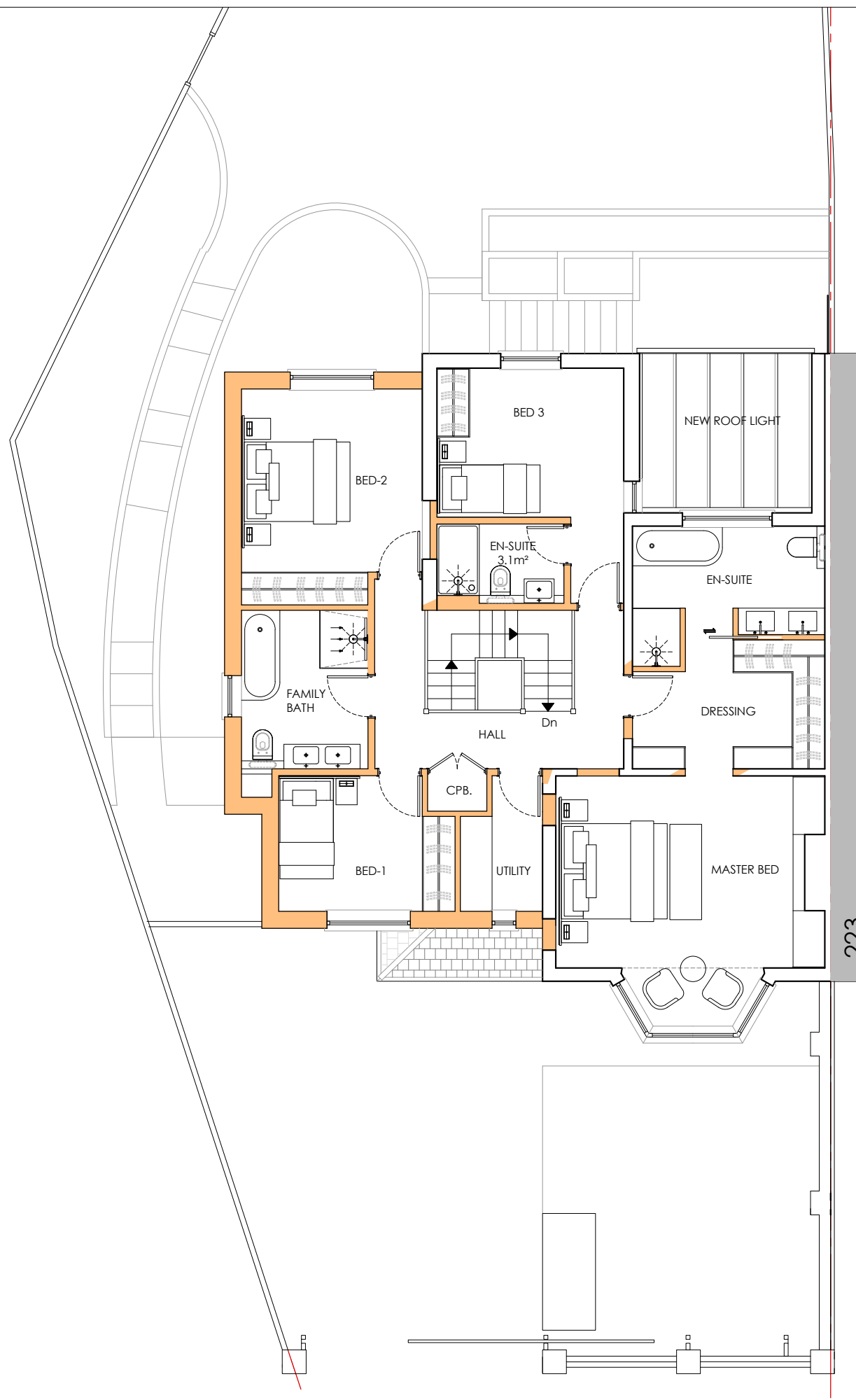
2 FIRST FLOOR PLAN PROPOSED 1:100
