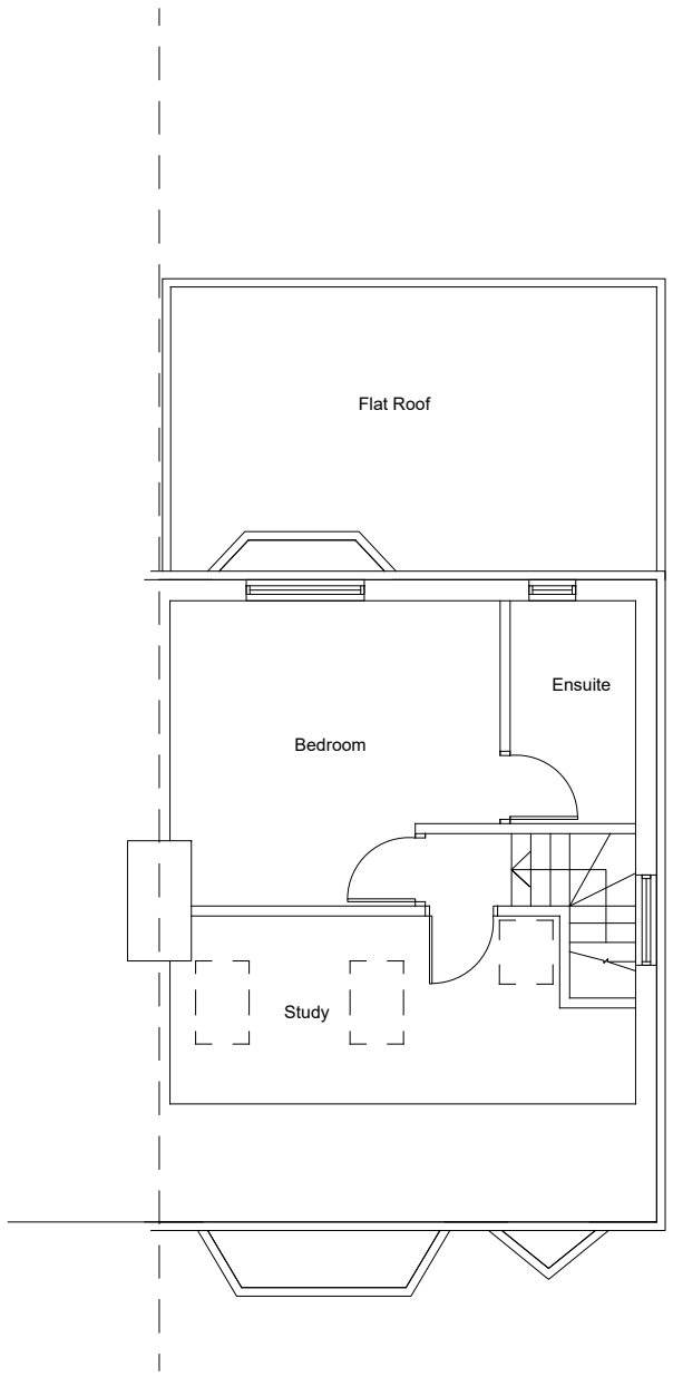
PROPOSED LOFT PLAN 1:100
