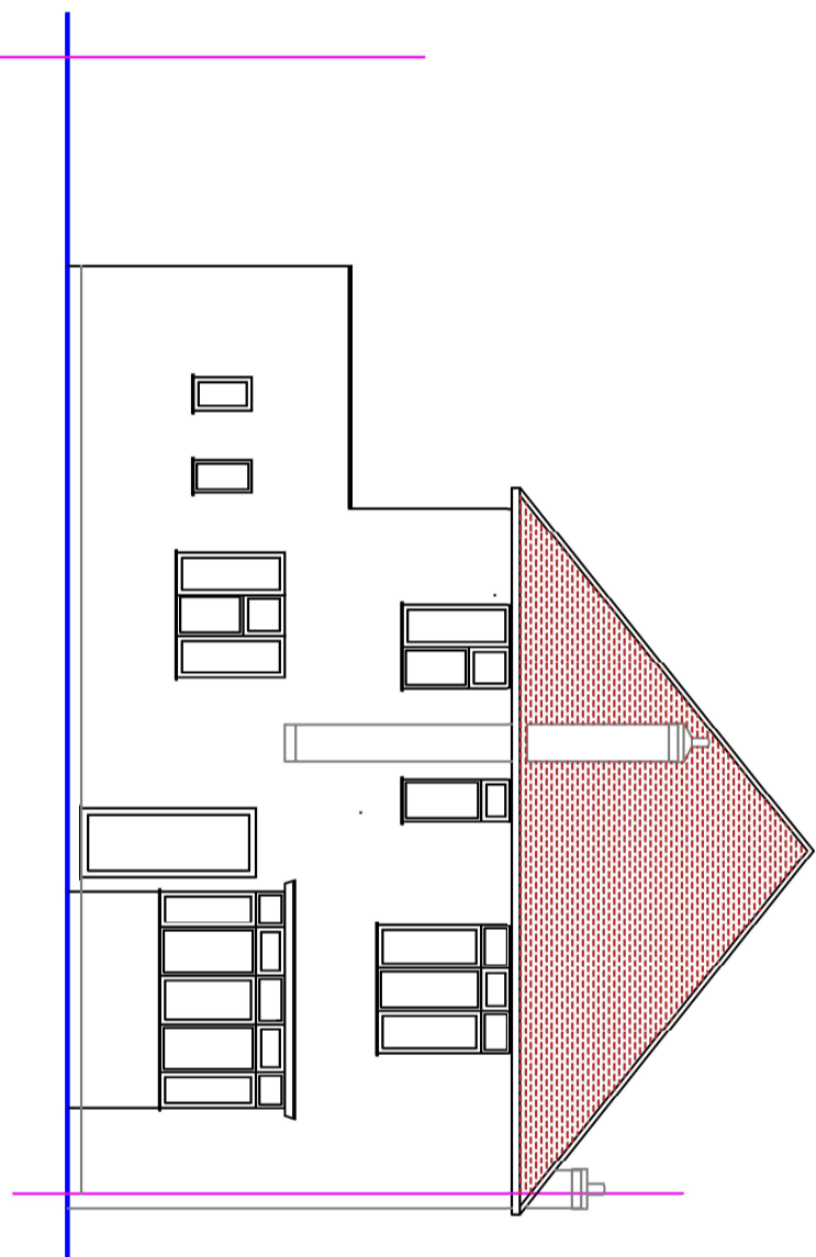
REAR ELEVATION (Existing)
