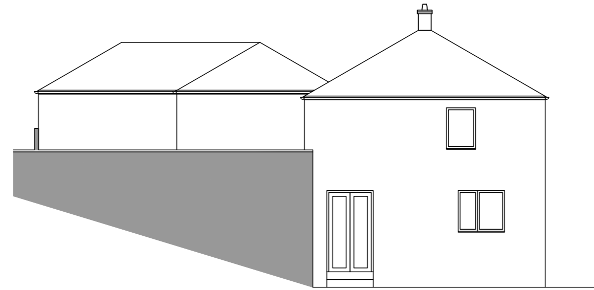
Proposed Elevation
