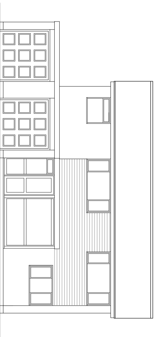
EXISTING FRONT ELEVATION 1:100
