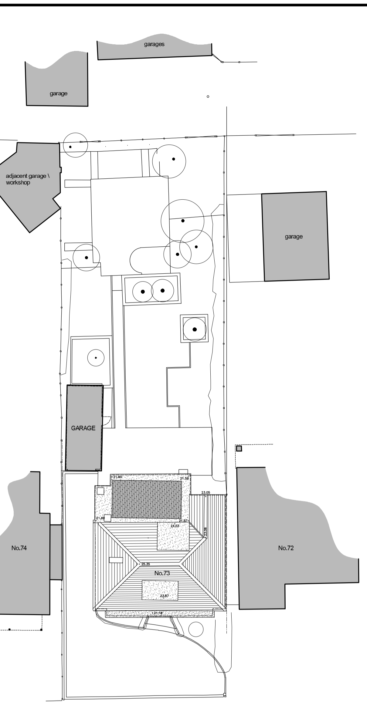
SITE BLOCK PLAN 1:200 @ A1
