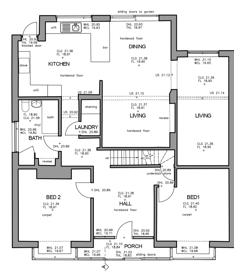
GROUND FLOOR PLAN 1:100 @ A1
