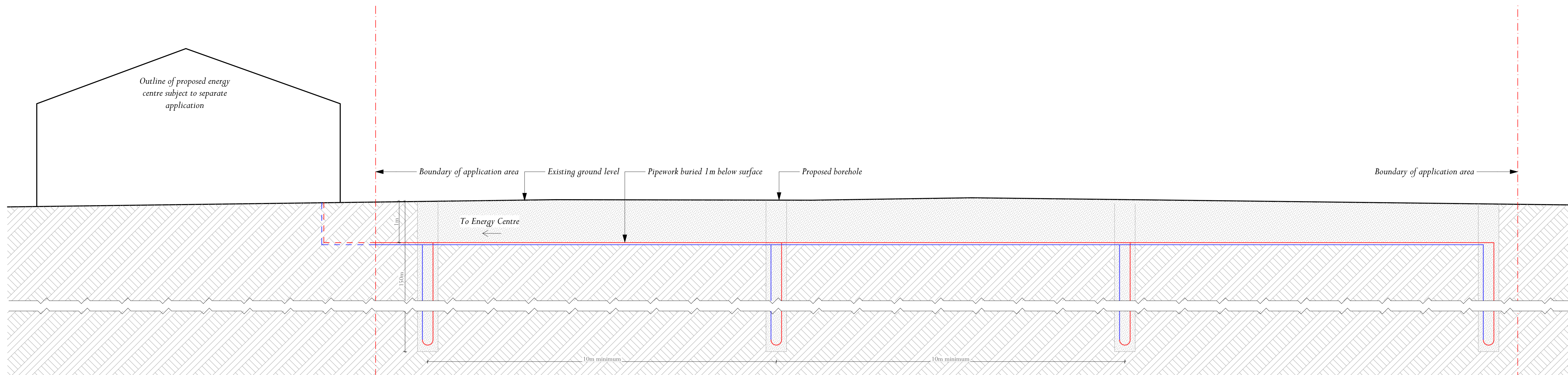
GSHP BOREHOLES SECTION B
