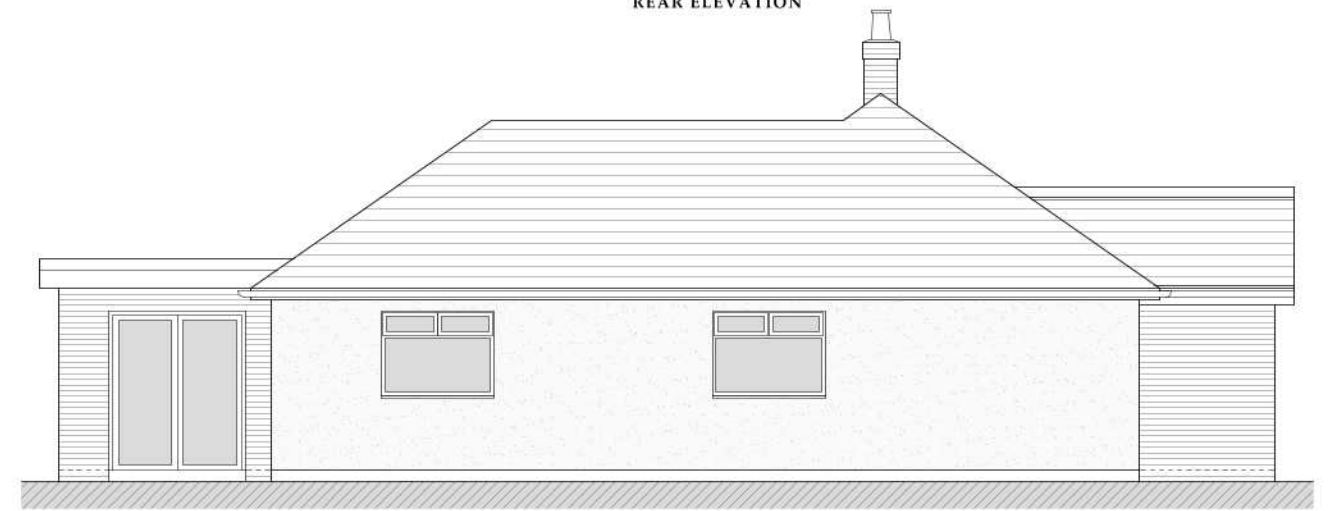
SIDE ELEVATION
