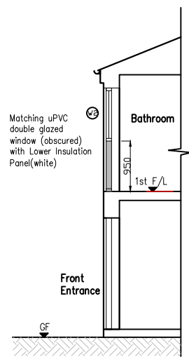
PROPOSED ELE. 'BB'
